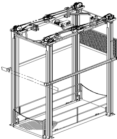
Figure I-3.1-3 Four-Post Design
