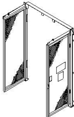
Figure I-3.9.2-2 Biparting, Double-Swing Hinged Gates
