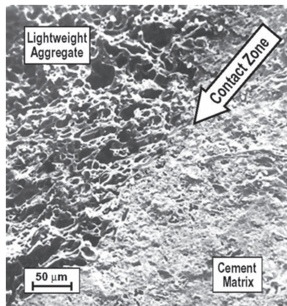
Fig. 6.3.2—Micrograph of contact zone.
