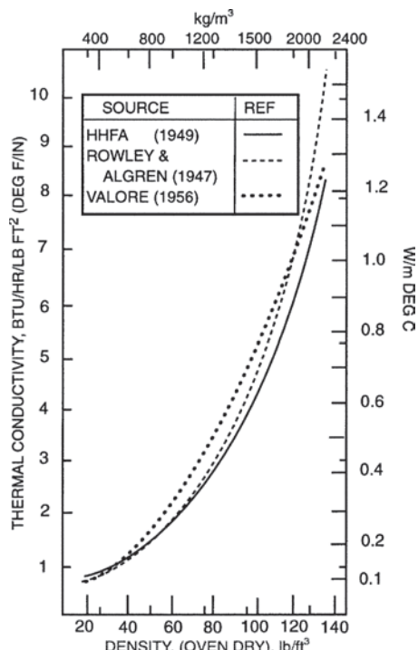
Fig. 5.12.1—Relation of average thermal conductivity k values of concrete in oven-dry condition to density (Valore 1980).
