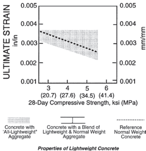
Fig. 5.7—Ultimate strain.
