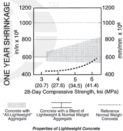
Fig. 5.9.2—Drying shrinkage: steam-cured concrete.
