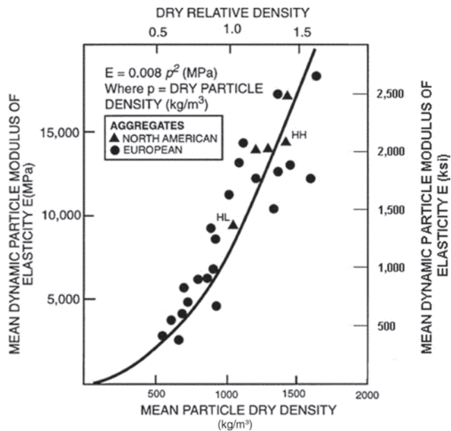
Fig. 3.3.8—Relationship between mean particle density and mean dynamic modulus of elasticity for particles of LWAs (Bremner and Holm 1986).
