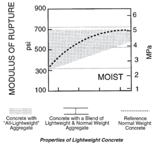
Fig. 5.4.2a—Modulus of rupture: normally cured concrete.
