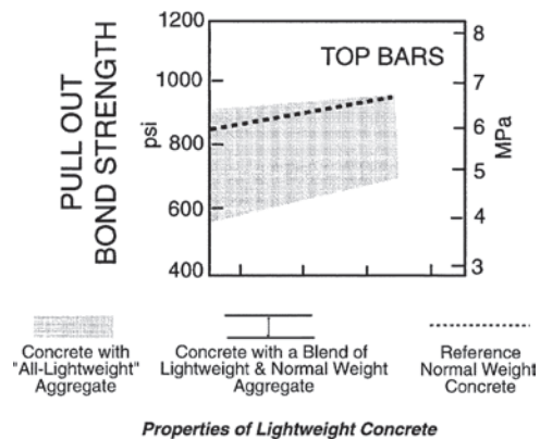
Fig. 5.10—Bond strength: pullout tests.
