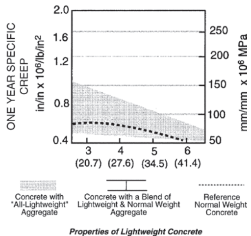
Fig. 5.8.3—Creep: steam-cured concrete.
