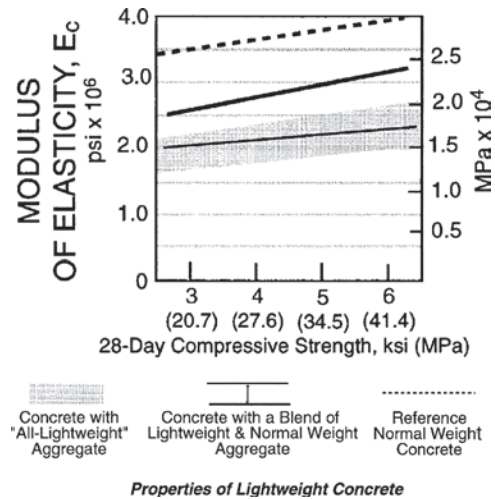
Fig. 5.5—Modulus of elasticity.
