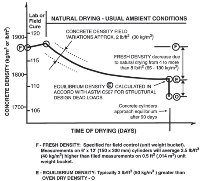
Fig. 5.3.2—Concrete density versus time of drying for structural lightweight concrete (Holm 1994).
