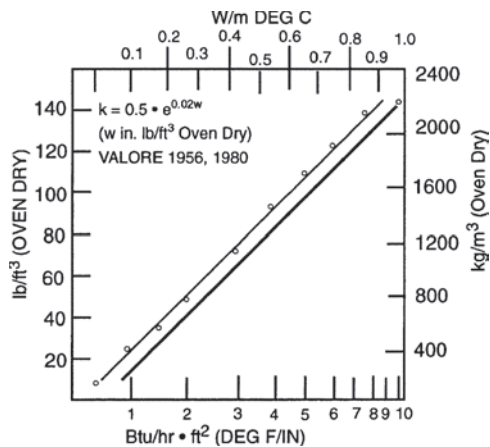
Fig. 5.12.1.3—Relation of average k values of concrete to dry density (Valore 1980).
