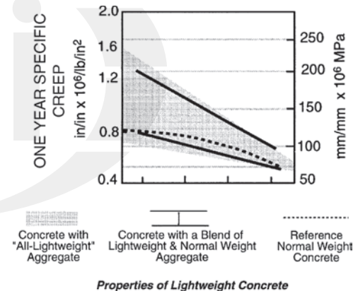
Fig. 5.8.2—Creep: normally cured concrete.
