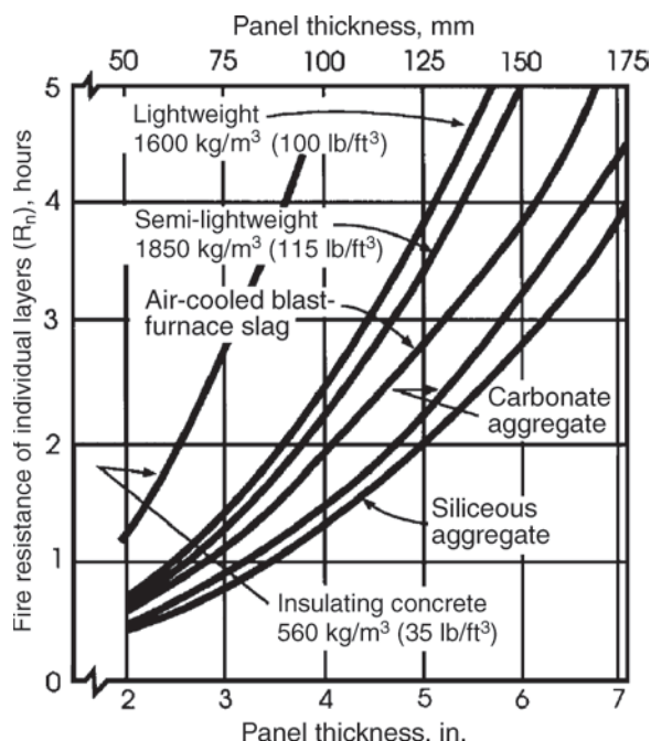
Fig. 5.13—Fire endurance (heat transmission) of concrete slabs as a function of thickness for naturally dried specimens (ACI 216.1).
