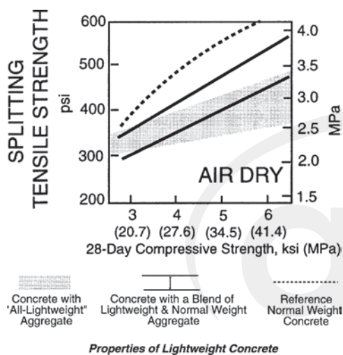
Fig. 5.4.1.2—Splitting tensile strength: air-dried concrete.
