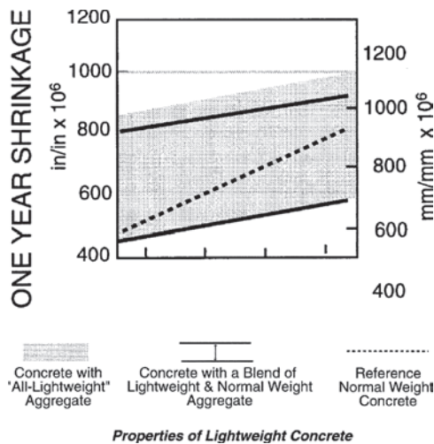
Fig. 5.9.1—Drying shrinkage: normally cured concrete.
