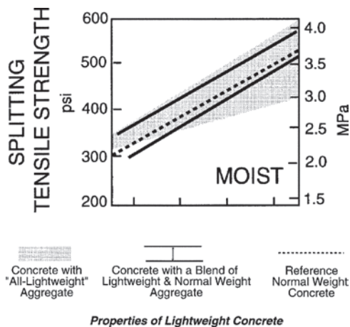
Fig. 5.4.1.1—Splitting tensile strength: moist-cured concrete.
