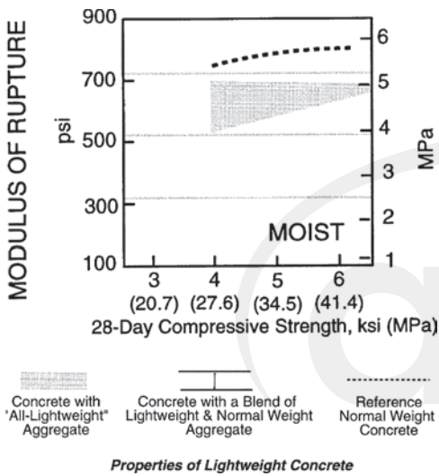
Fig. 5.4.2b—Modulus of rupture: steam-cured concrete.
