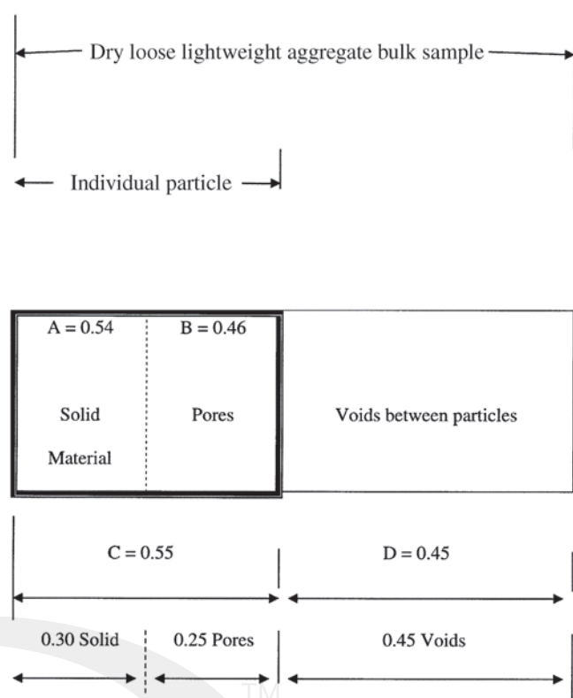
Fig. 3.3.5—Representation of solids, pores, and voids in LWA.
